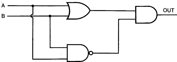
C. XOR gate using OR, AND, and NAND gates.
